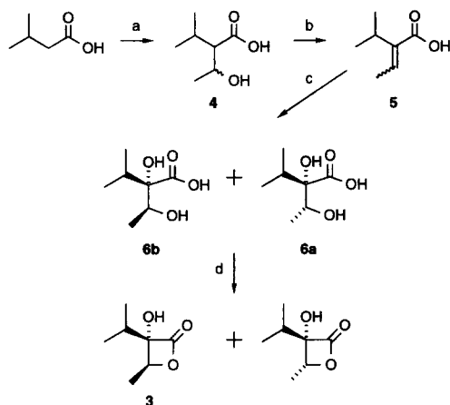
Figure 4. Synthesis of 2-hydroxy-2-(1-methylethyl)-3-butanolides (relative configurations). (a) 2 equiv n -BuLi, \text{CH}_3\text{CHO} ; (b) \text{P}_2\text{O}_5 ; (c) \text{K}_3\text{Fe}(\text{CN})_6 , \text{OsO}_4 ; \text{CH}_3\text{SO}_2\text{Cl} , \text{Na}_2\text{CO}_3 .
