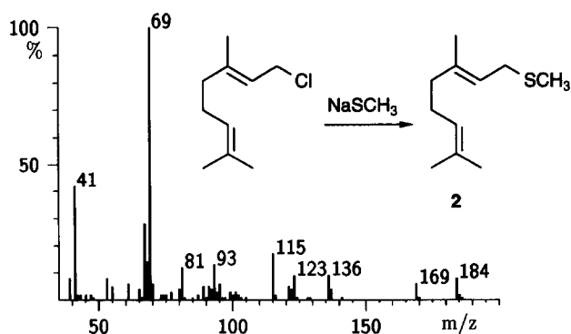
Figure 3. Mass spectrum and synthesis of ( E )-3,7-dimethyl-2,6-octadienyl methyl thioether (geranyl methyl thioether, 2).
