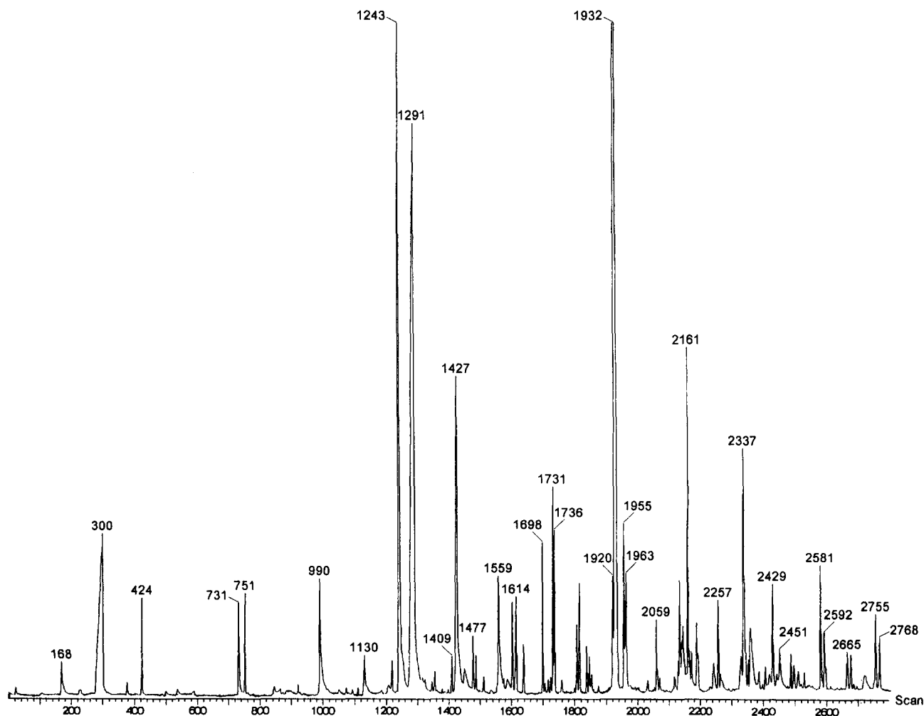
Figure 2. Total ion chromatogram of a hairpencil extract from I. leuconoe . The scan numbers are used for identification of compounds in Tables 1 and 2.
