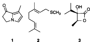
Figure 1. Pheromone components of I. leuconoe .
