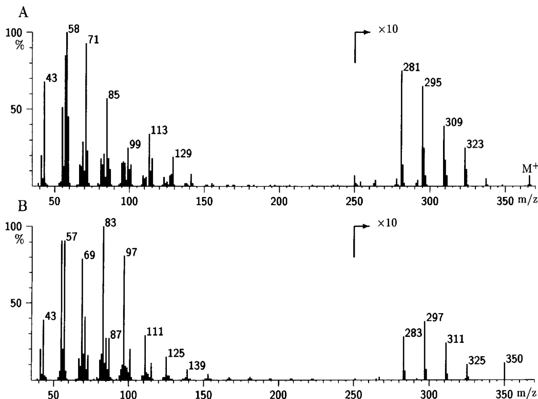
Figure 7. Mass spectrum of (A) a mixture of 4-, 5-, 6- and 7-pentacosanones and (B) a mixture of 4-, 5-, 6- and 7-pentacosanols.
