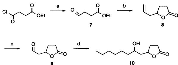
Figure 5. Synthesis of 6-hydroxy-4-dodecanolide. (a) \text{H}_2 , Pd/C, lutidine; (b) \text{CH}_2=\text{CHCH}_2\text{ZnCl} , DMSO, then \text{H}^+ ; (c) \text{O}_3 , then \text{H}_2 , Pd/C; (d) \text{C}_6\text{H}_{13}\text{MgBr} .
