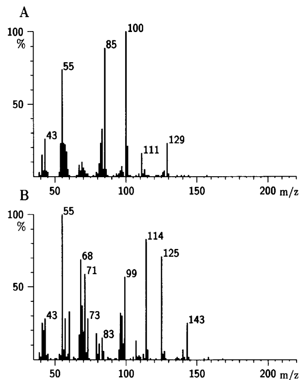
Figure 6. Mass spectrum of (A) 6-hydroxy-4-dodecanolide ( 10 ) and (B) 7-hydroxy-5-dodecanolide.
