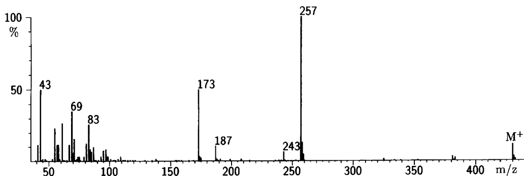
Figure 8. Mass spectrum of a mixture of DMDS adducts of 9- and 14-tricosen-2-, 3-, 4-, 5-, 6- or 7-ones, in which the 14-enones dominated.
